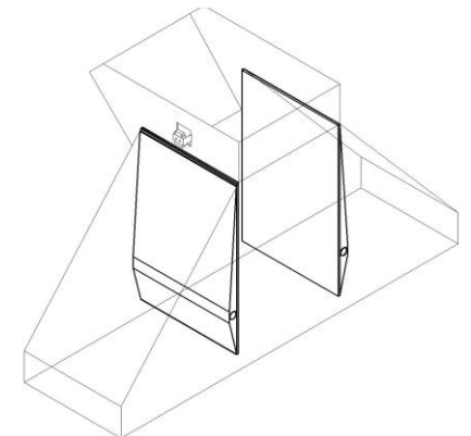
Diverter Flaps BOLD Centre Position with Flared Extension shown
