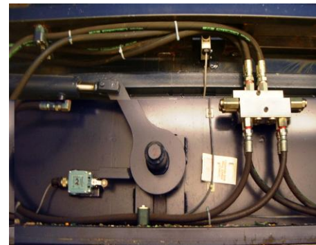
Sorter CAM & Hydraulic Connections
